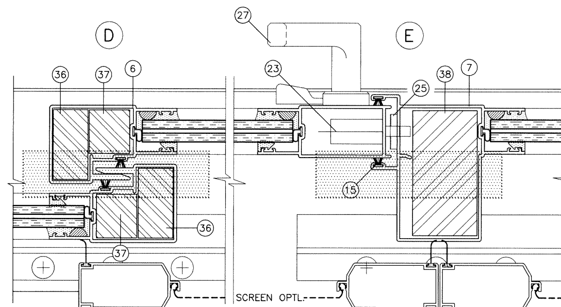
HEAVY REINFORCING AT EXTERIOR/INTERIOR INTERLOCK & ASTRAGAL STILES
