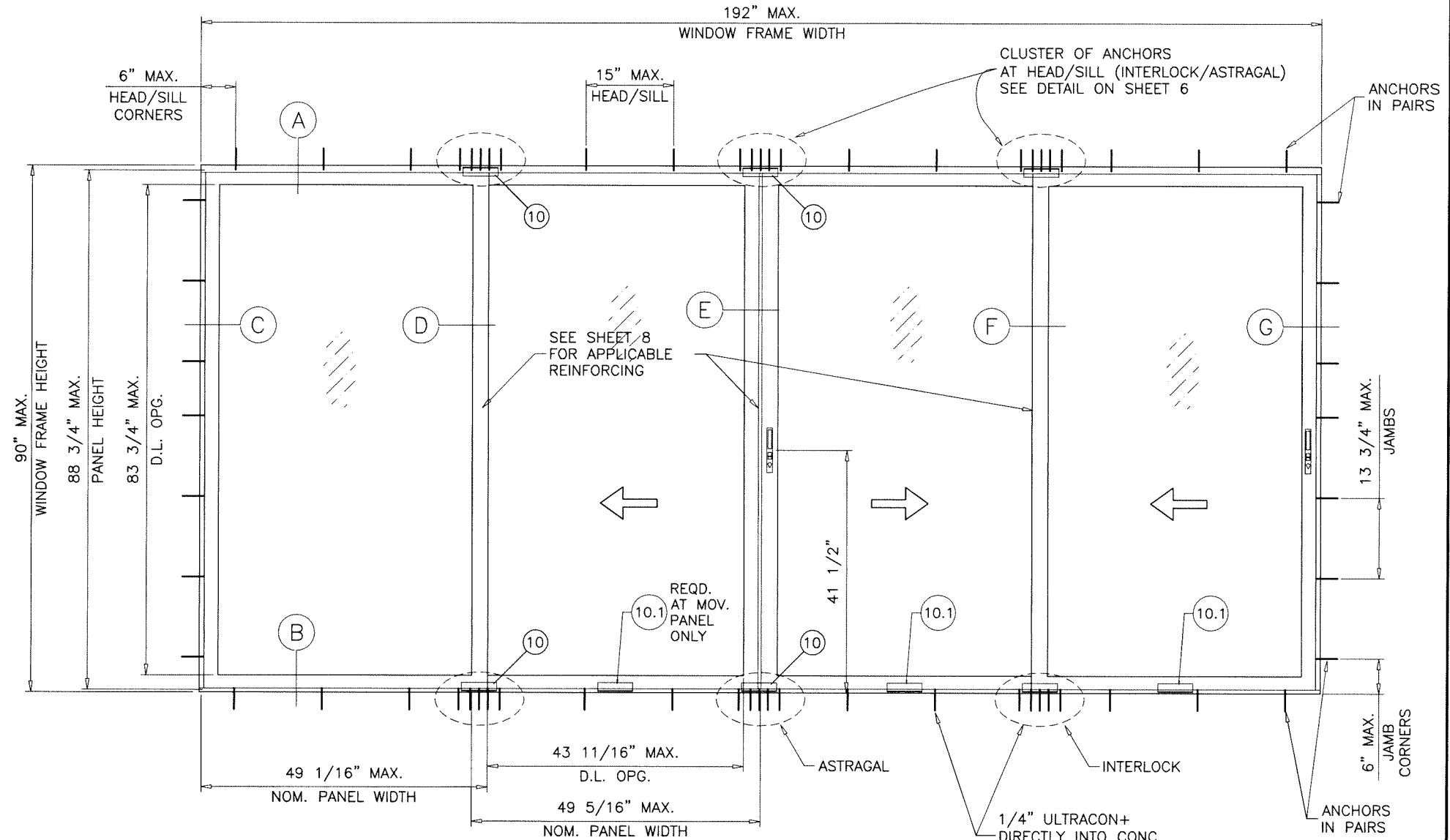
TYPICAL ELEVATION
