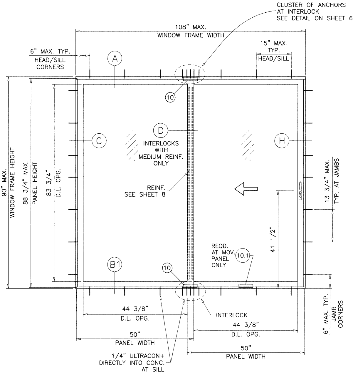
TYPICAL ELEVATION (OX) (SHOWN)
